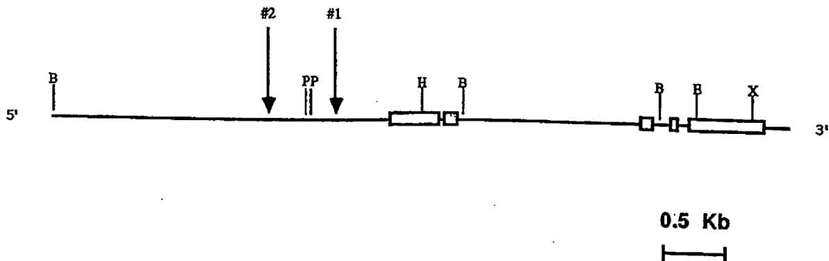
Fig 2. Relationship of chromosome 5 breakpoints to the IL-3 gene. This figure shows the two cloned breakpoints (arrows) in relation to the normal IL-3 gene. 10 One breakpoint occurred at position -462 and the other at -934 (arrows). In both circumstances, the translocations resulted in a head-to-head joining of the IgH gene and the IL-3 gene, leaving the mRNA and protein coding regions of the IL-3 gene intact. Boxes denote the five IL-3 exons; restriction enzymes are (B) Bam HI, (P) Pst I, (H) Hpa I, (E) Eco RI, and (X) Xho I.
